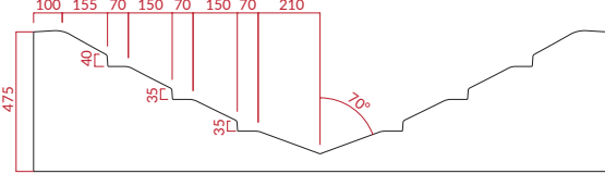
SECTION C
