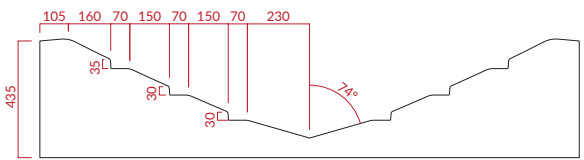
SECTION B
