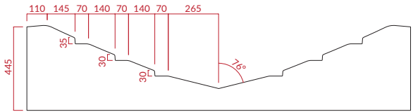
SECTION A
