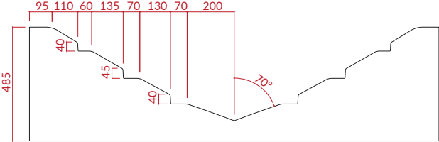
SECTION C
