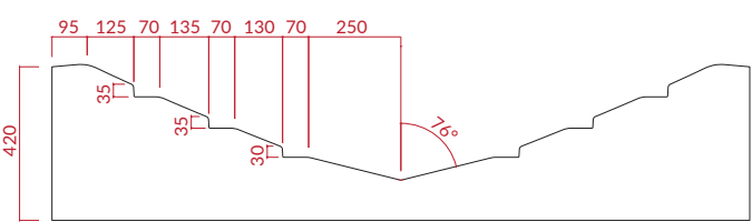
SECTION A
