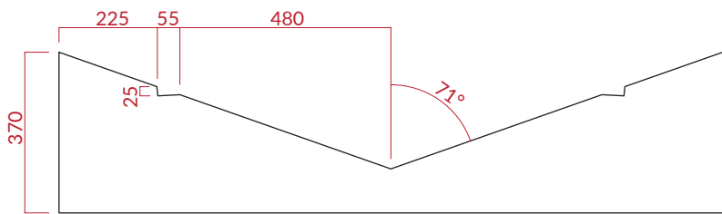
SECTION A
