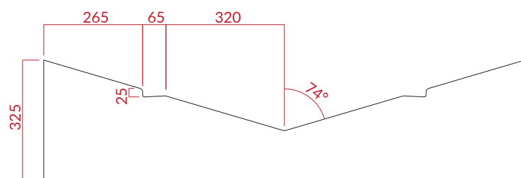
SECTION A
