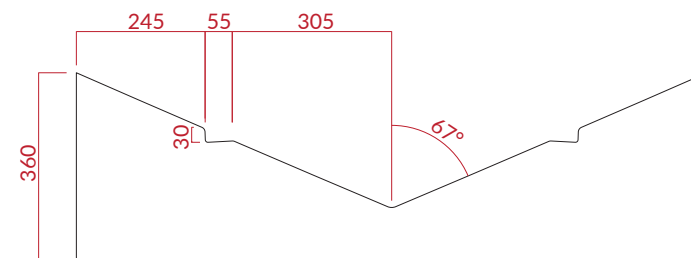
SECTION B
