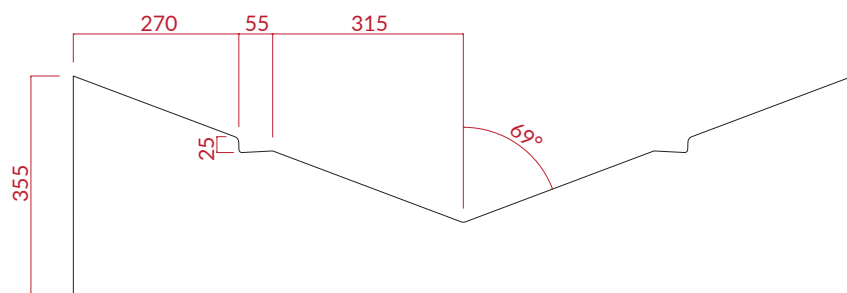
SECTION A
