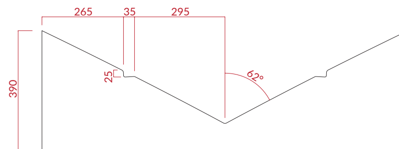
SECTION B
