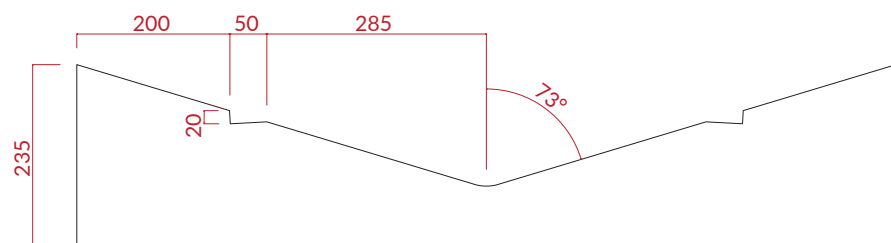
SECTION A
