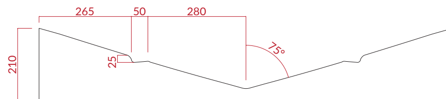
SECTION B
